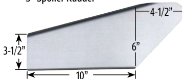
5" Spoiler Rudder
