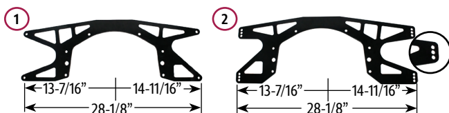
5/8" OFFSET CHEVY
