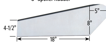
8" Spoiler Rudder
